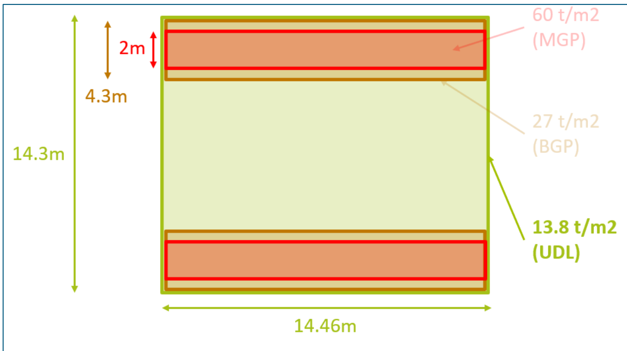
Figure 2-10 Liebherr LR 11350 P1800 pressure calculation
