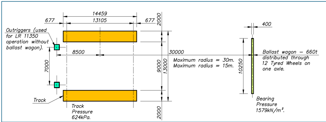
Figure 2-9 Liebherr LR 11350 P1800 crane
